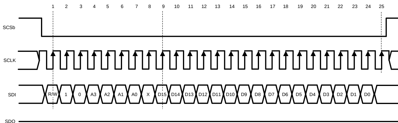
Figure 43. Serial Data Protocol - Write Operation
