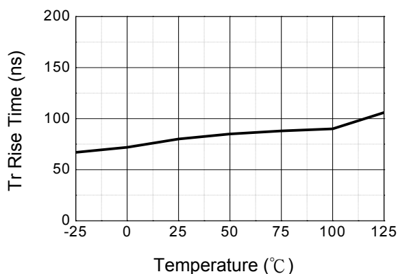
Figure 3. Tr Rise Time vs Temperature
