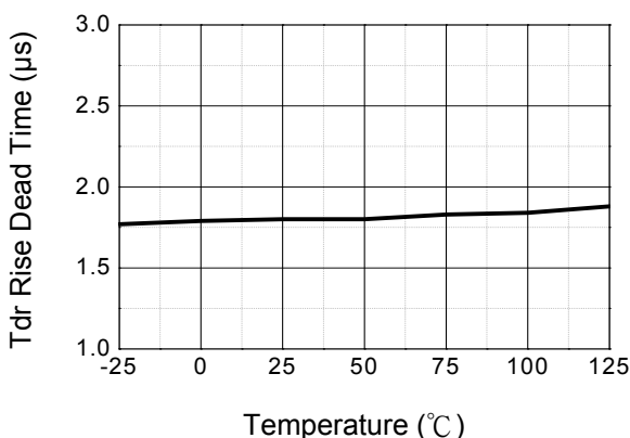
Figure 5. Tdr Rise Dead Time vs Temperature
