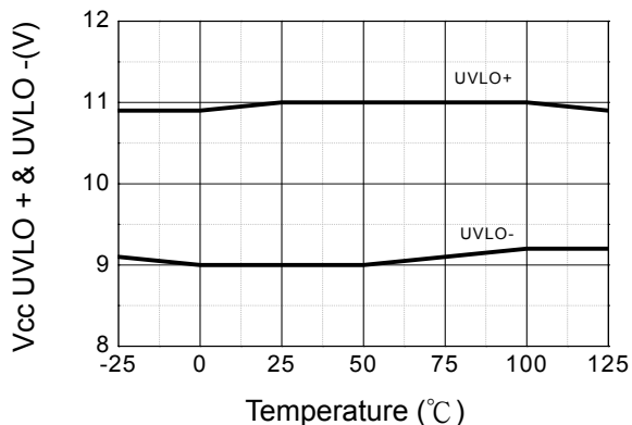
Figure 1. Vcc UVLO+ & UVLO- vs Temperature
