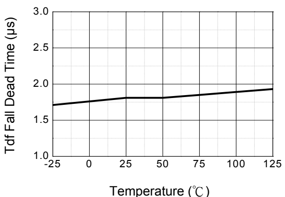
Figure 6. Tdf Fall Dead Time vs Temperature
