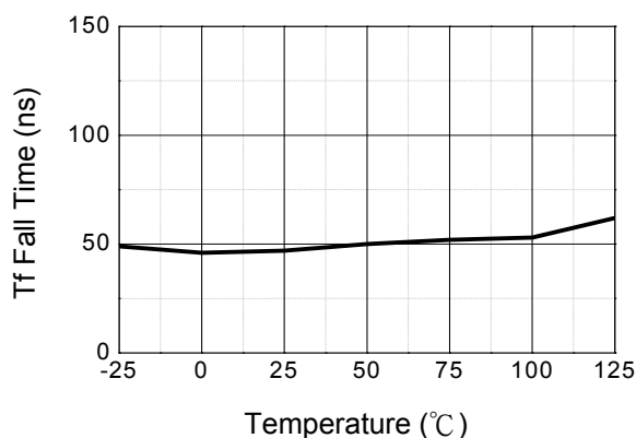
Figure 4. Tf Fall Time vs Temperature
